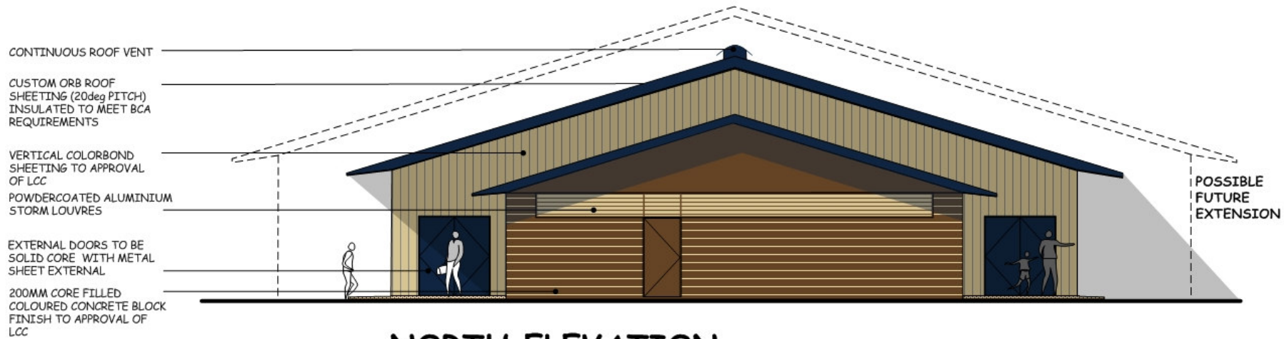
NORTH ELEVATION
