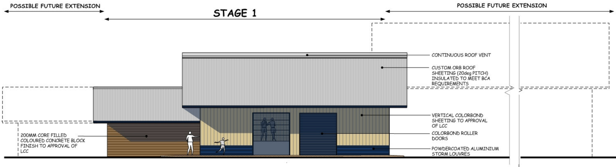
WEST ELEVATION
